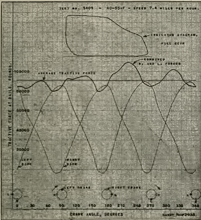
TRACTIVE FORCE CURVES, FULL GEAR, 11S LOCOMOTIVES, CYLINDERS 30 1/2 X 32 INS., STEAM PRESSURE 250 LBS.
